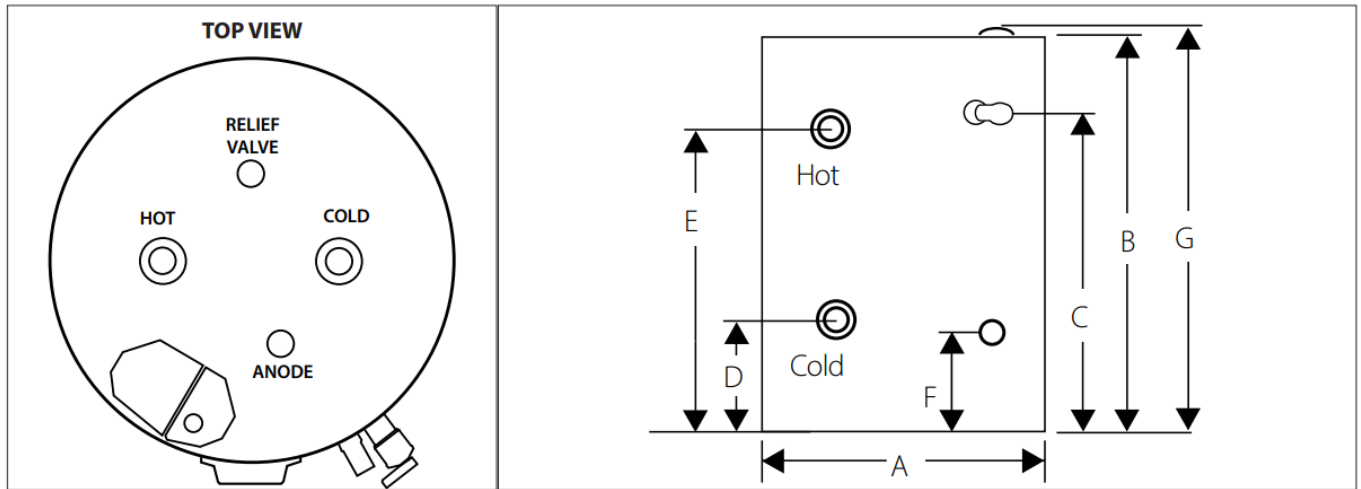
Figure 2 - Dimensional Drawing
