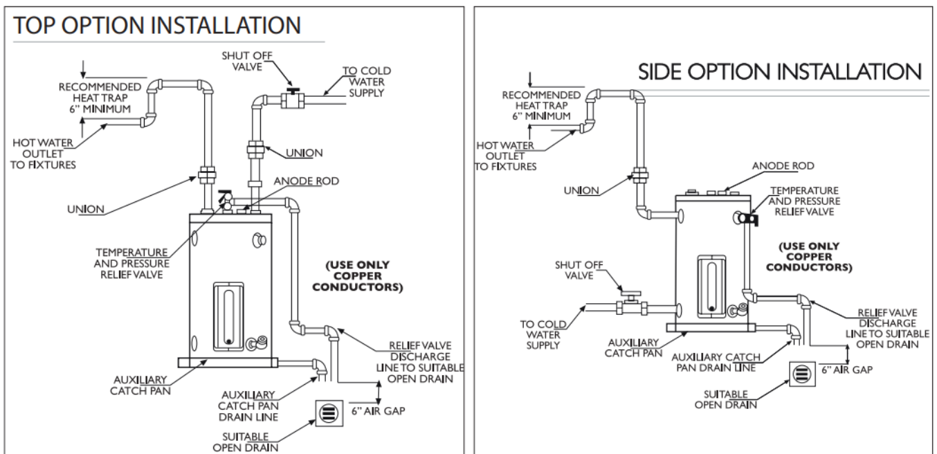
Figure 4 - Piping Details - NOTE: Drawings are meant to demonstrate system piping concept. Heat traps are optional but recommended.
