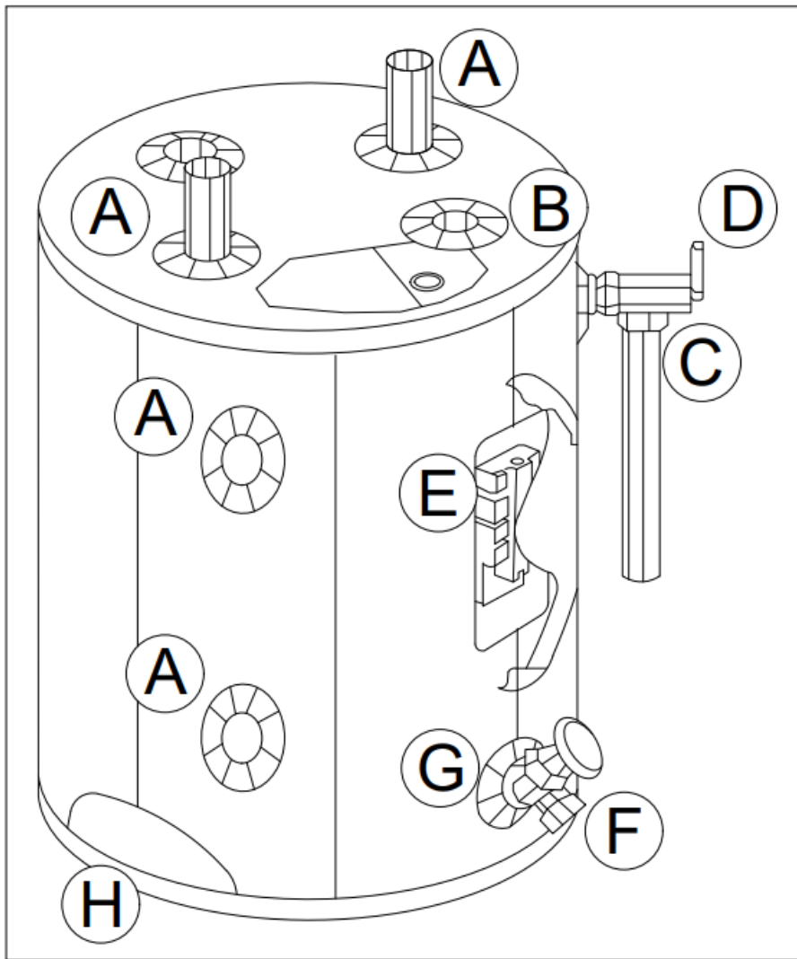
Figure 7 - Leakage Checkpoints
