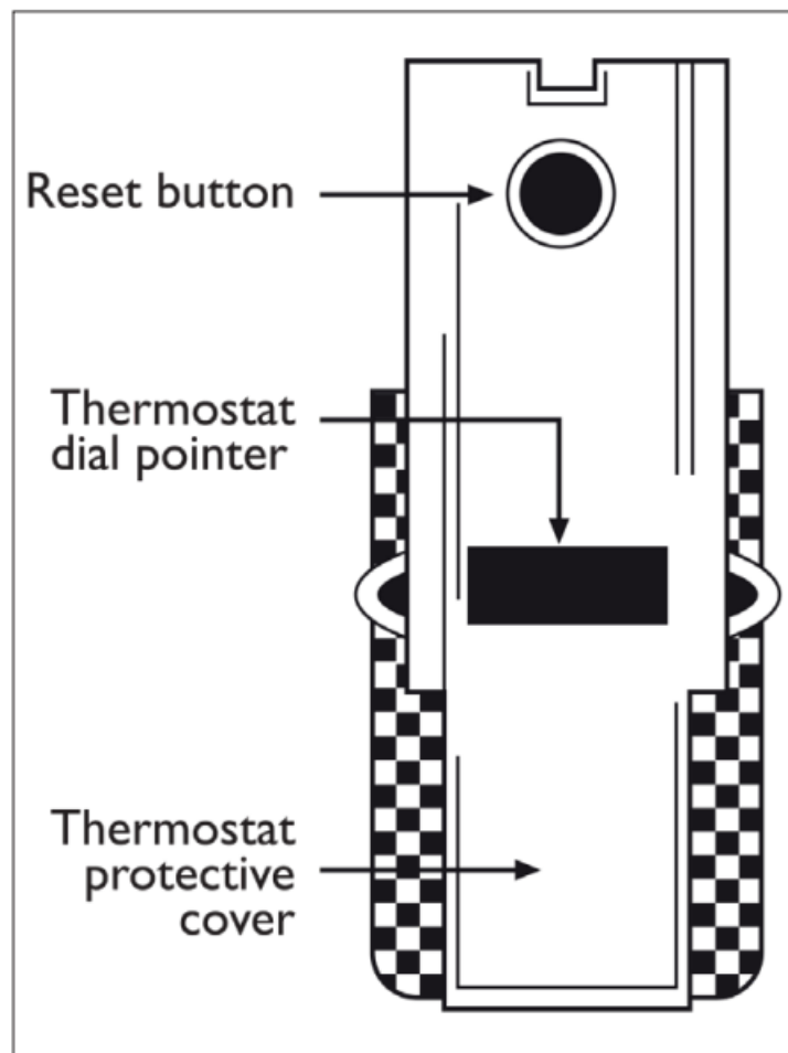
Figure 6 - Thermostat Detail
