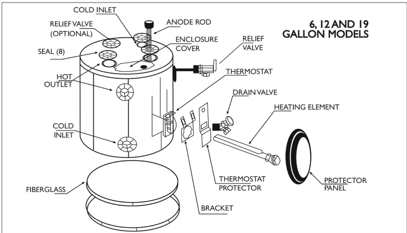
Figure 8 - Replacement Parts - Non-Simultaneous Operation
