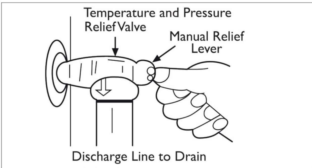
Figure 3 - T&P Relief Valve Operation
